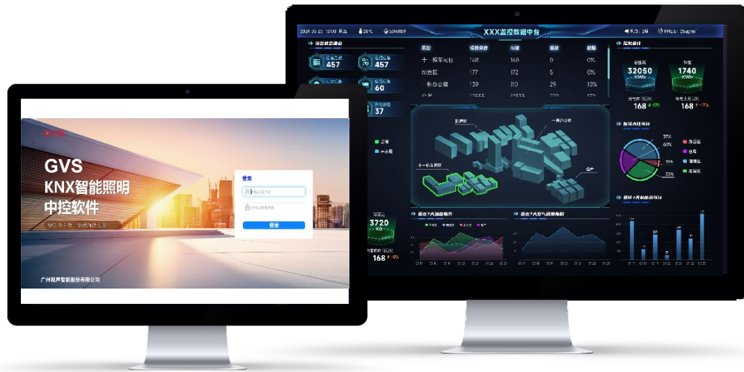
Login Interface
